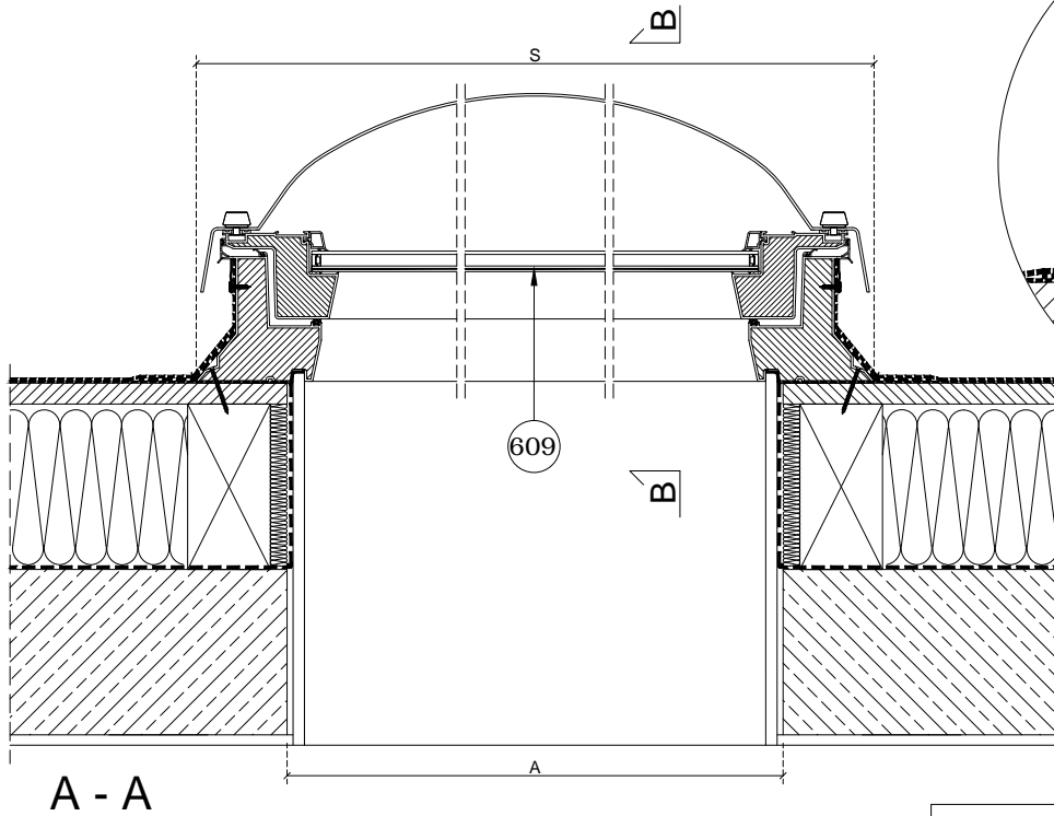
609-DMC-C P2 Flat Roof Window, manually opened, with transparent dome
